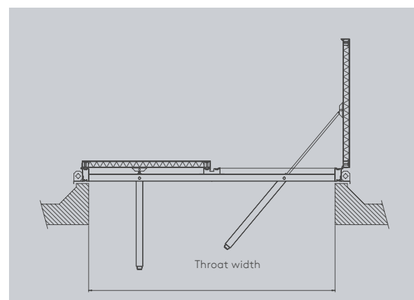
Cross Section
